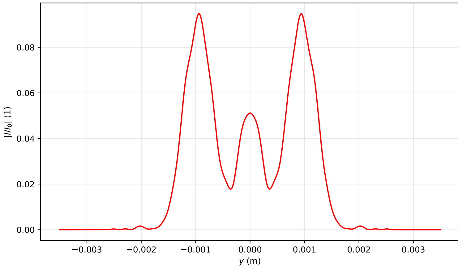
Intensity profile I(x=0, y, z=2.627)/I_0 , \text{Pin}=7.0\text{Pcr} , artificial time
